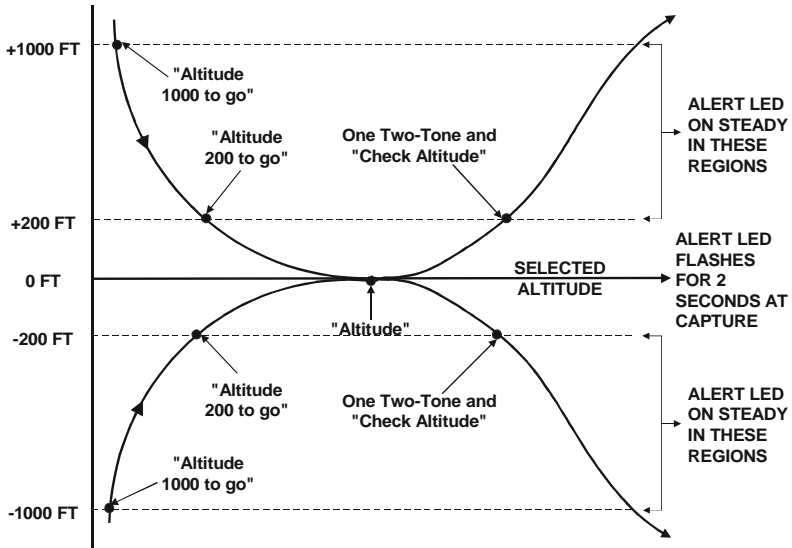
Fig. 4-2. Altitude Selector / Alerter Annunciation Flight Profile
