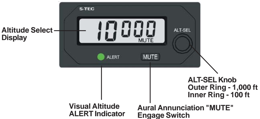
Fig. 3-1. Altitude Selector / Alerter Quick Reference
