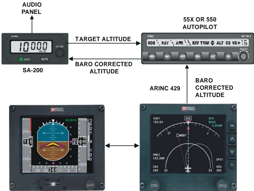
Fig. 2-2. SA-200 Altitude Selector/Alerter Block Diagram (With MAGIC EFIS)
